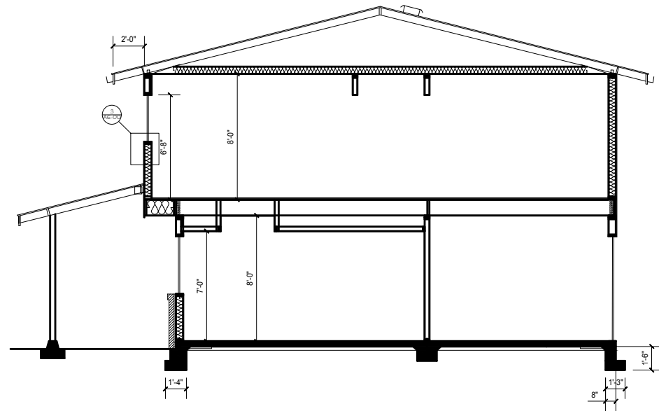
2 Building Section Scale: 1/8"=1'-0"
